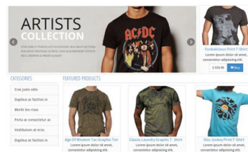
(/page/e-commerce)
