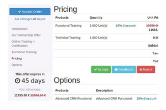
(/page/quote-builder)
